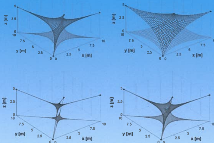
Cable network equilibrium configurations
